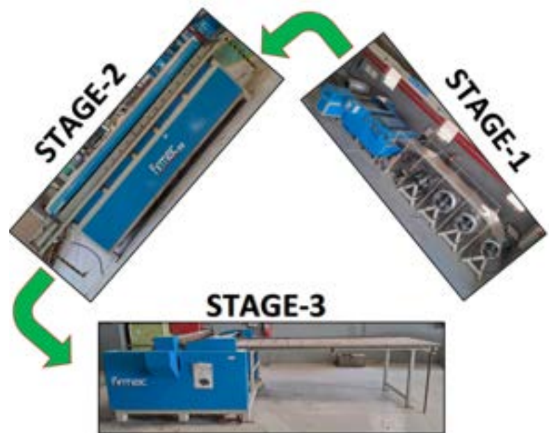
Firmac MDF 1500 Modular Duct Forming System (Stage 1 to 3)
